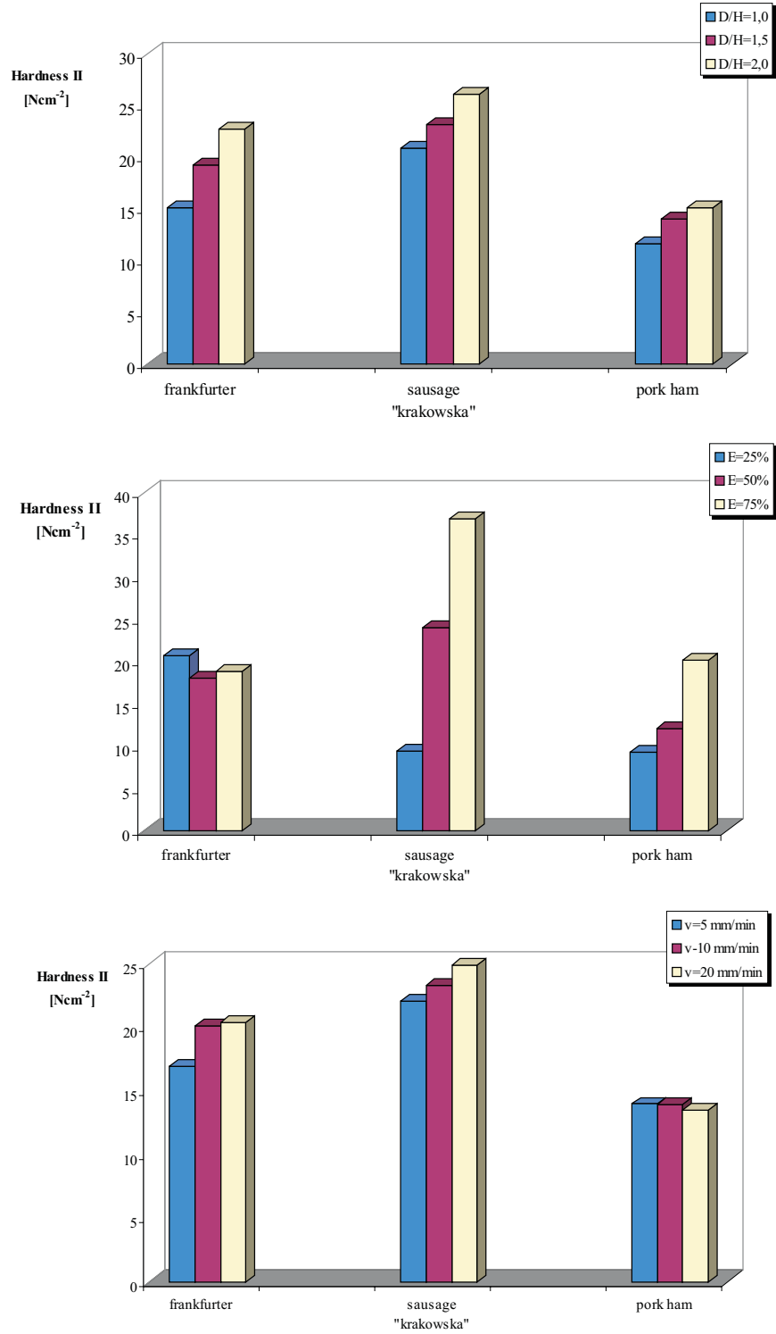
Fig. 2. Influence of sample size, sample deformation degree and sample loading speed on the hardness II values.
