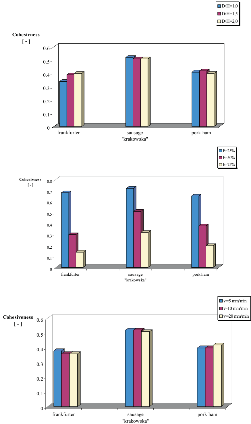
Fig. 4. Influence of sample size, sample deformation degree and sample loading speed on the cohesiveness values.
