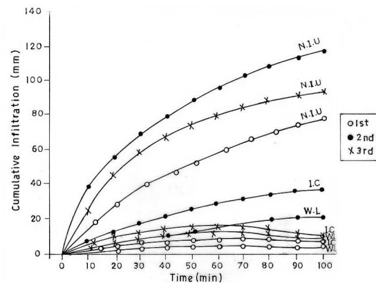
Fig. 2. Cumulative infiltration as a function of time for soils of three moisture regimes (NIU – non-irrigated upland, IC – irrigated cultivated, WL – waterlogged, 1st-2nd-3rd refer to seasons).
