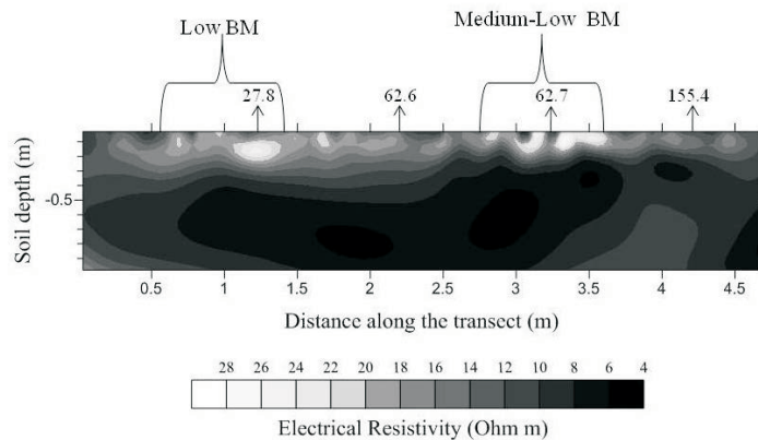
Fig. 2. 2D-electrical resistivity tomogram generated in Transect A; areas comprised within the braces show areas of low and medium-low rocket biomass (BM) values at visual assessment. Black arrows indicate sampling locations and corresponding fresh biomass values.
