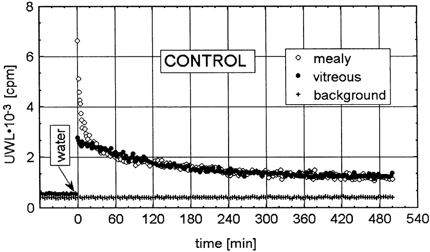
Fig. 1. Comparison of UWL from the control samples (not moistened) of mealy and vitreous wheat grain.
