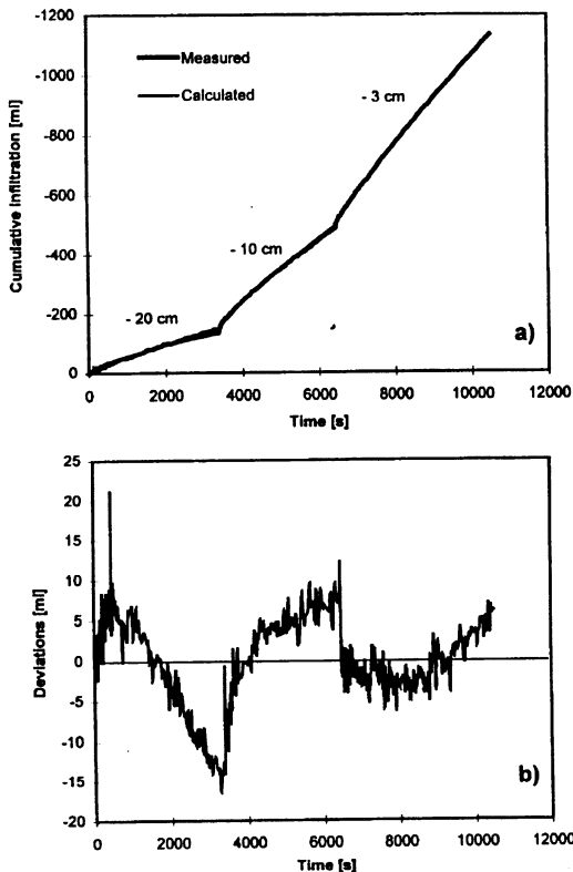
Fig. 1. Tension disc infiltrometer experiment; Run 1: a) measured and fitted cumulative infiltration curves versus time, b) deviations between measured and fitted cumulative infiltration versus time. The fitted curve was obtained by minimizing the objective function \phi(I, \theta_p) .
