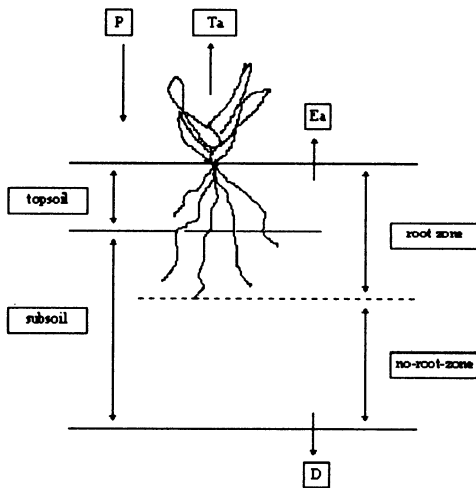
Fig. 1. Basic compartments of the soil-plant system for ACCESS-I.
