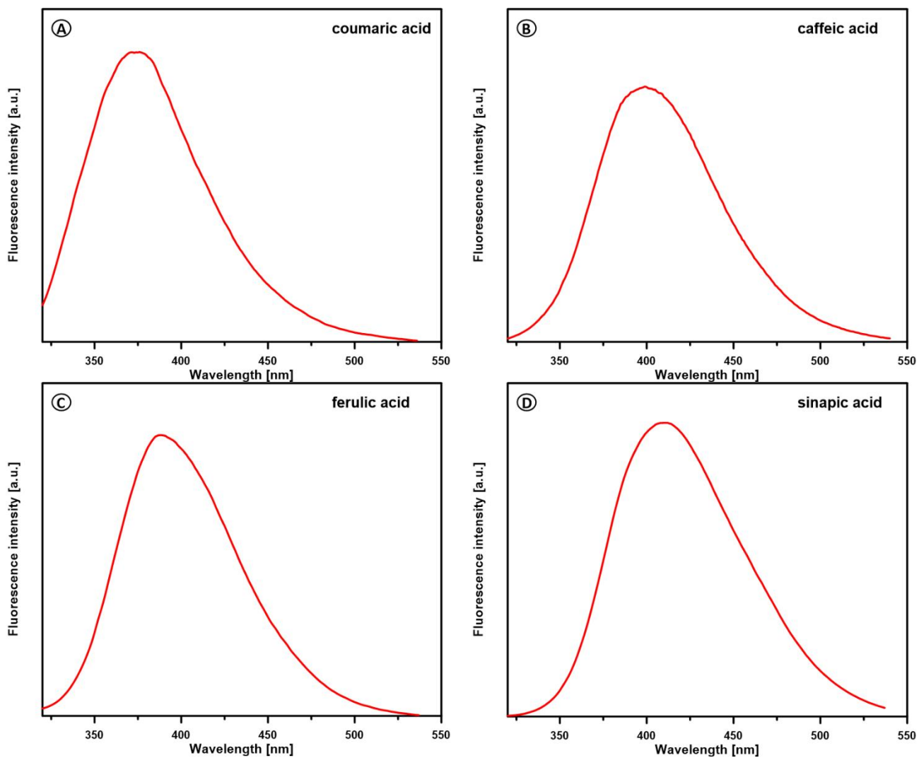
Fig. S2. Fluorescence emission spectra of phenolic acids in ethanol solution.
