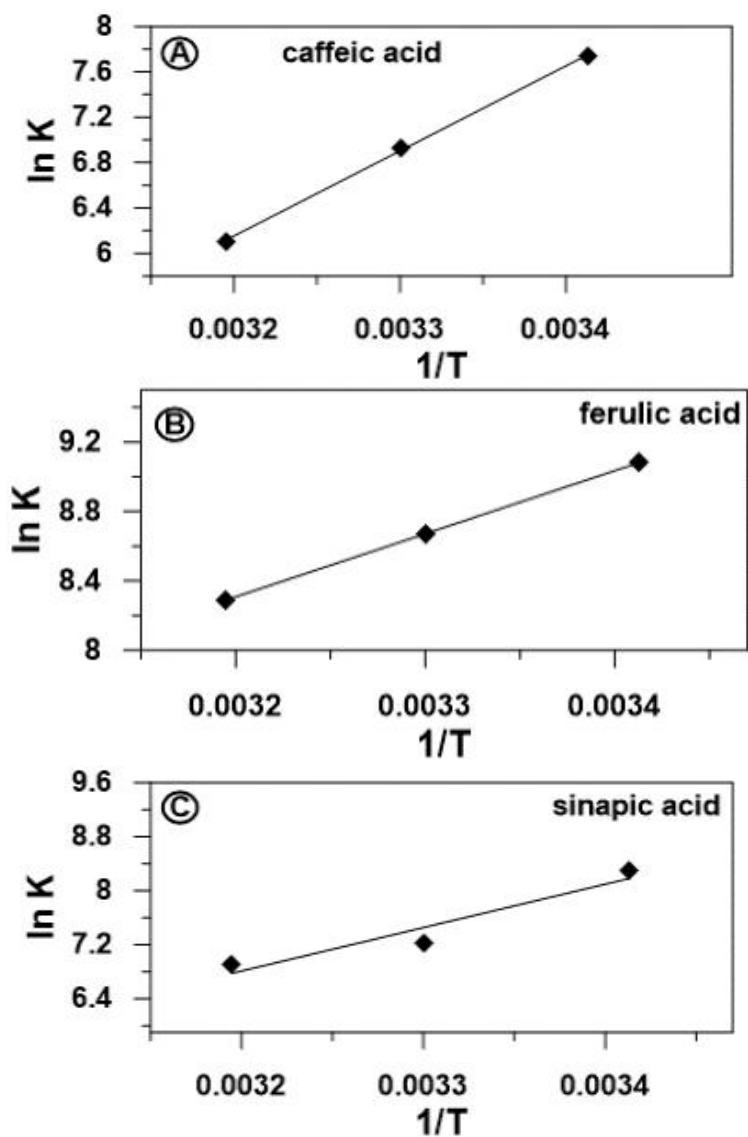
Fig.S1 Van't Hoff plots of \ln K as a function of 1/T (K) for the binding of gliadin to phenolic acids.
